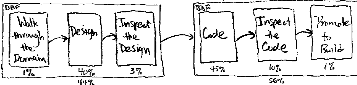
Figure 6-6. DBF/BBF milestone with schedule percentages.
