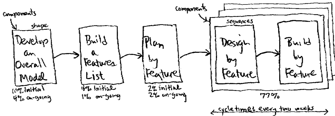
Figure 6-5. FDD processes with schedule percentages.
