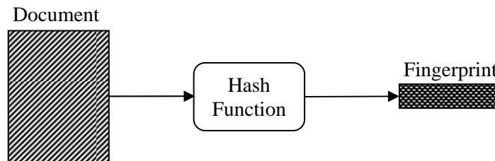
Figure 2 Hash function
