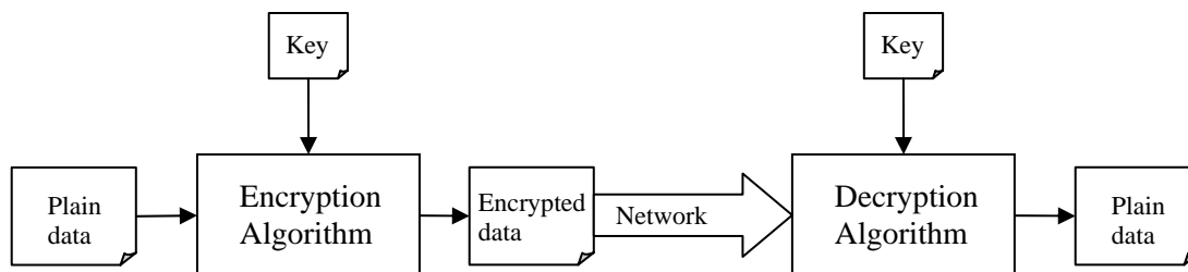
Figure 1 Data encryption/decryption
