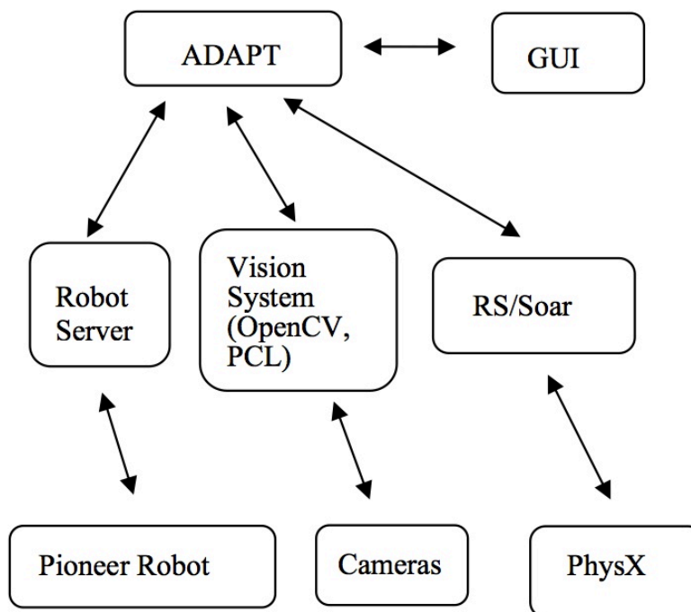
Figure 1. ADAPT architecture.
