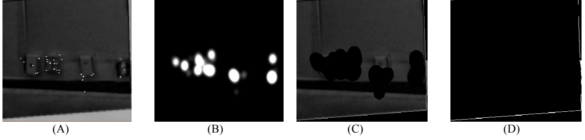
Figure 5: Absolute difference of warped real and synthetic images with overlaid match points (A) and match mediated difference mask (B) calculated from (A). Match mediated absolute difference (C) and thresholded difference (D).
