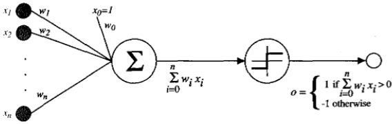
FIGURE 4.2 A perceptron.
