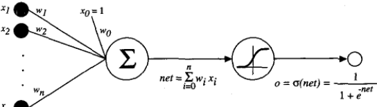
FIGURE 4.6 The sigmoid threshold unit.
