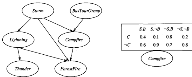
FIGURE 6.3 A Bayesian belief network. The network on the left represents a set of conditional independence assumptions. In particular, each node is asserted to be conditionally independent of its nondescendants, given its immediate parents. Associated with each node is a conditional probability table, which specifies the conditional distribution for the variable given its immediate parents in the graph. The conditional probability table for the Campfire node is shown at the right, where Campfire is abbreviated to C , Storm abbreviated to S , and BusTourGroup abbreviated to B .
