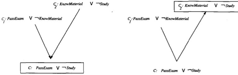
FIGURE 10.2 On the left, an application of the (deductive) resolution rule inferring clause C from the given clauses C_1 and C_2 . On the right, an application of its (inductive) inverse, inferring C_2 from C and C_1 .
