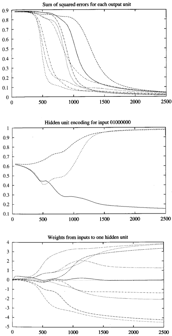
FIGURE 4.8 Learning the 8 \times 3 \times 8 Network. The top plot shows the evolving sum of squared errors for each of the eight output units, as the number of training iterations (epochs) increases. The middle plot shows the evolving hidden layer representation for the input string "01000000." The bottom plot shows the evolving weights for one of the three hidden units.
