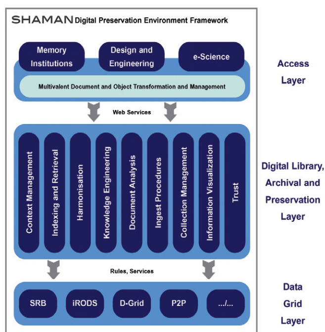
Figure 2: The informal and generic conceptual view for the SHAMAN architectural framework.
