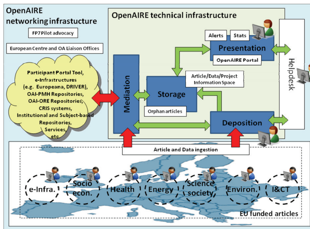
Figure 1: OpenAIRE infrastructure.
