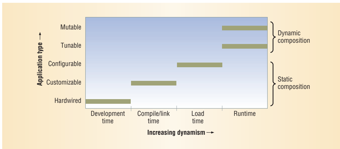
Figure 3. Classification for software composition using the time of composition or recomposition as a classification metric.
