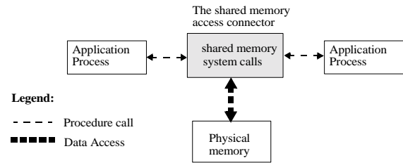
Figure 5. The shared memory access connector.
